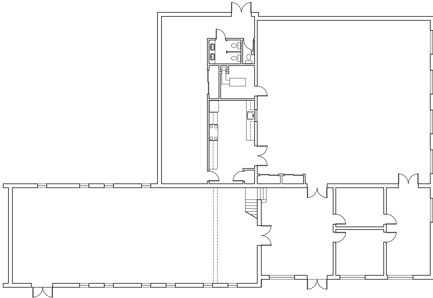
MADISON LUTHERAN CHURCH - EXISTING FLOOR PLAN
